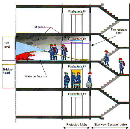
Figure A.1 — Fire adjacent to the protected lobby
